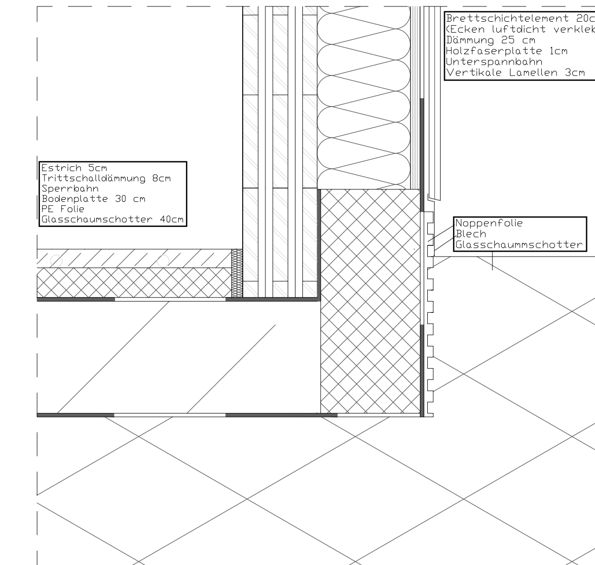
detail 3, 1:10
