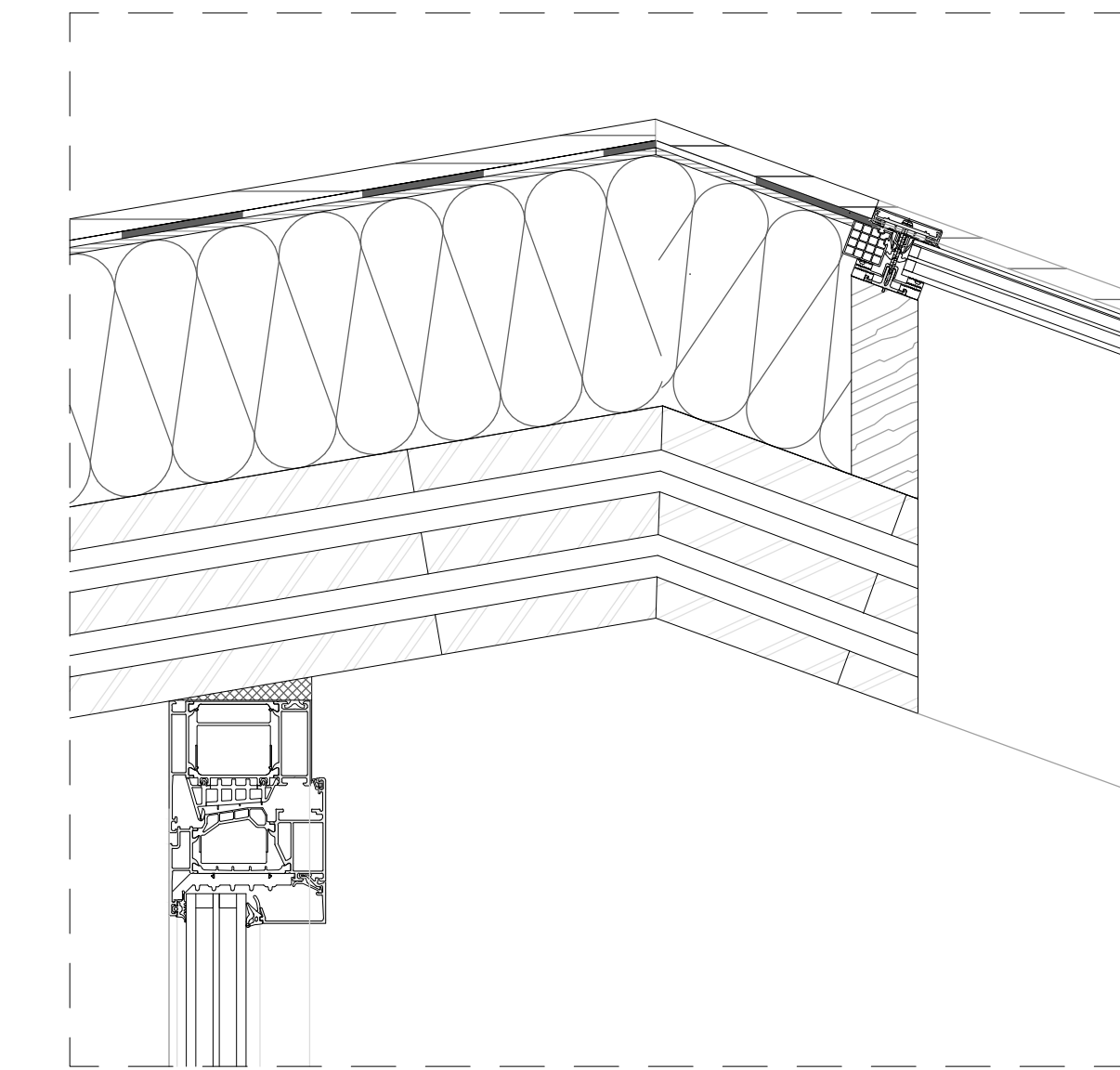
detail 1, 1:10
