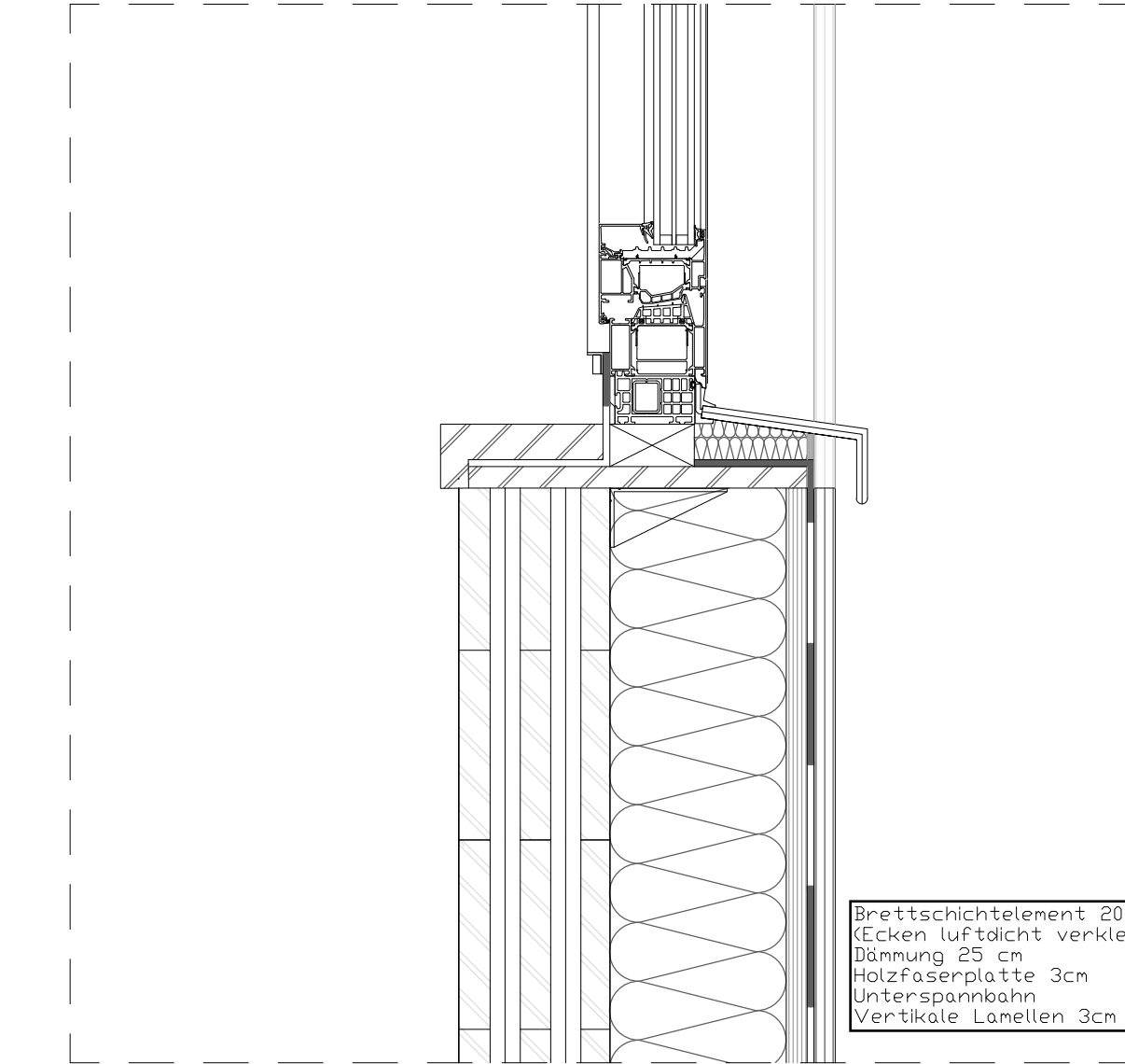
detail 2, 1:10
