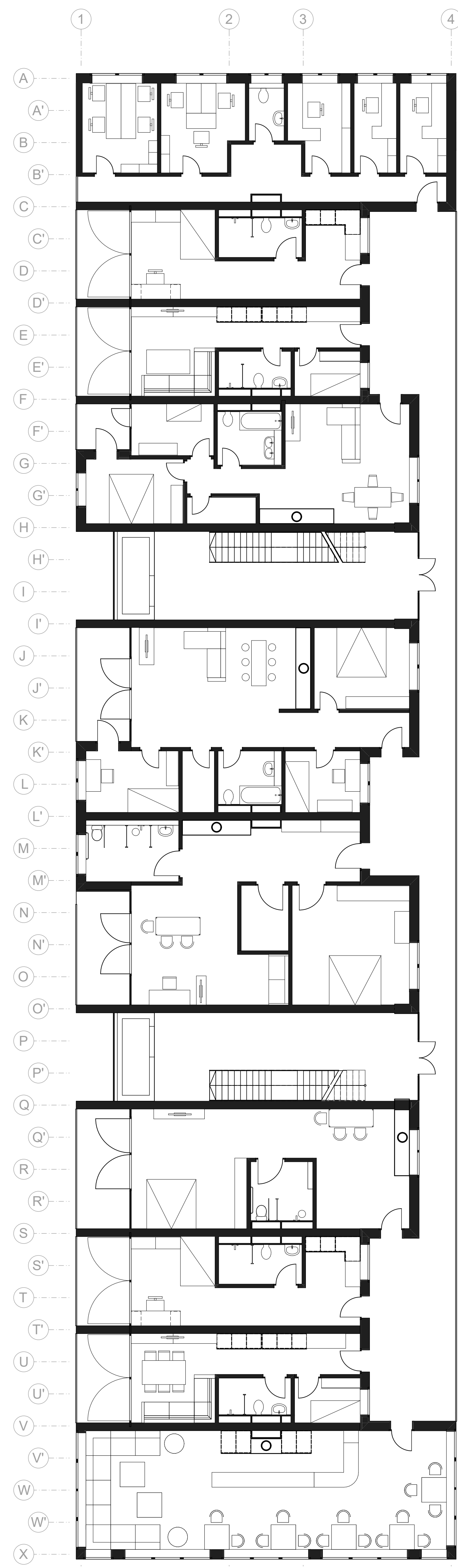
Grundriss 1.0G M1:100
