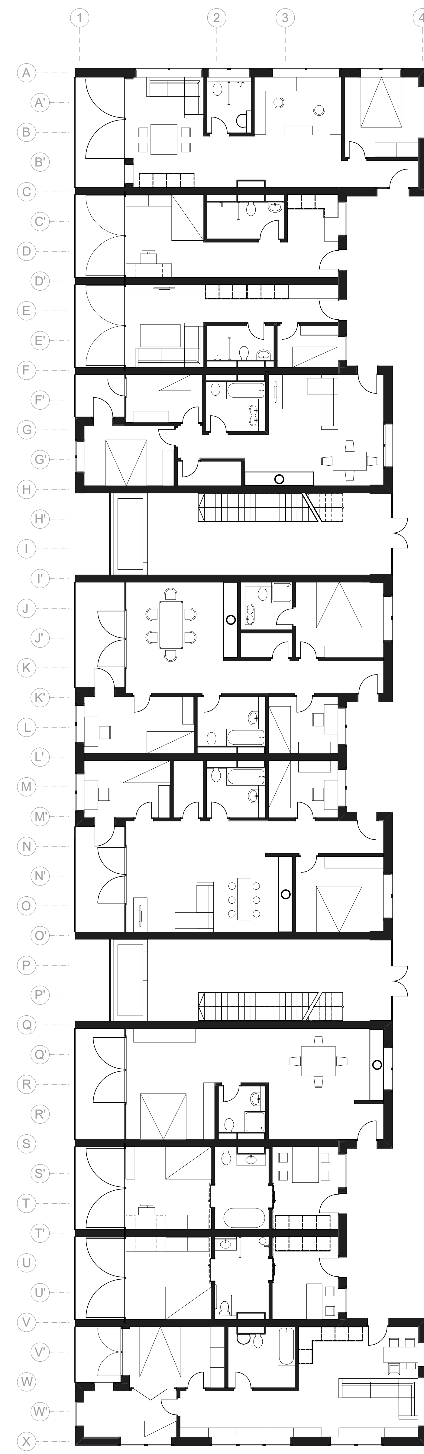
Grundriss 2.0G M1:100
